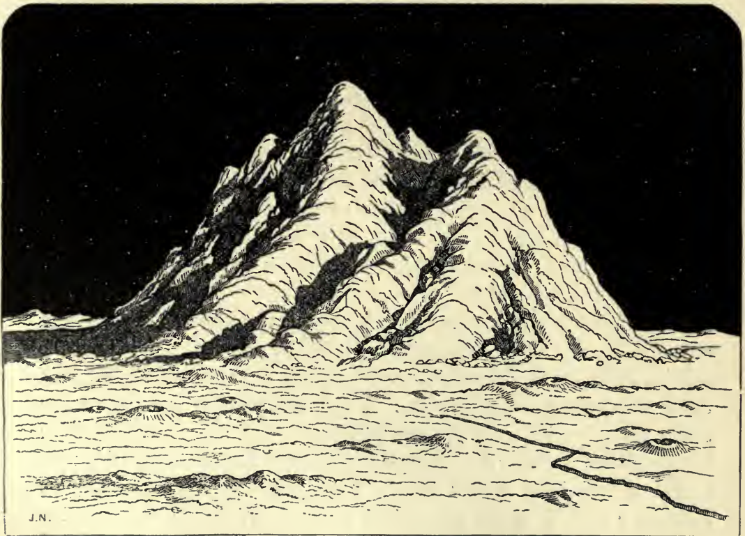
IDEAL SKETCH OF PICO AS IT WOULD PROBABLY APPEAR IF SEEN BY A SPECTATOR LOCATED ON THE MOON.
