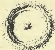
COPERNICUS. 46 Miles Diam r
