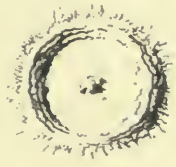
ERATOSTHNES. 33 Miles Diam r
