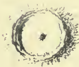
AGRIPPA. 30 Miles Diam r
