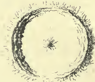
ALPHONS. 70 Miles Diam r
