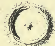
WERNER. 38 Miles Diam r
